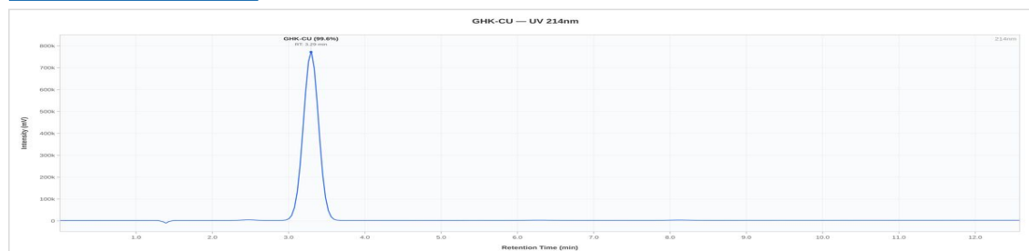
GHK-CU 100mg - 032026: UV Chromatogram
