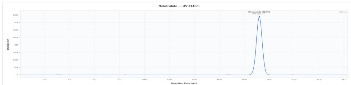
Retatrutide 20mg - 032026: UV Chromatogram
