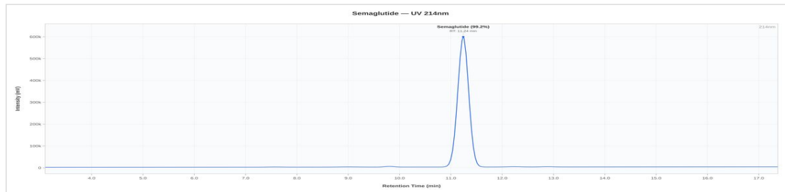
Semaglutide 10mg - 032026: UV Chromatogram
